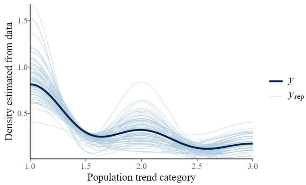
Fig. S2. Graphical posterior predictive check comparing empirical distribution of the observed data ( y , thick line) to the distribution of simulated data from the posterior predictive distribution of the model using 100 random draws ( y_{rep} , thin lines).
